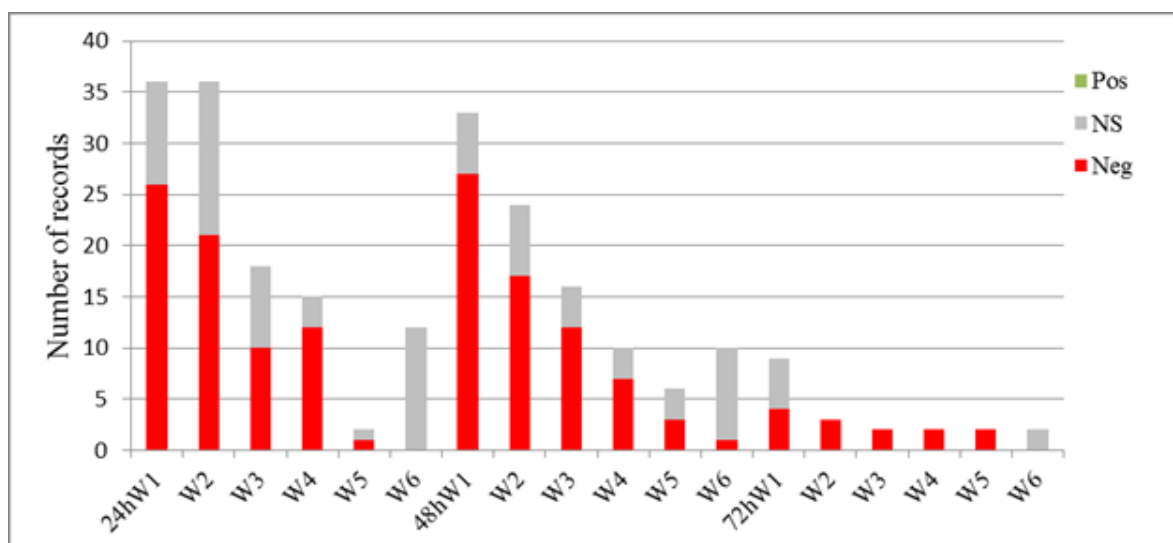
Figure 1 Results of QA of records including the effect of post-hatch food and water deprivation on body weight . The graph shows the number of records indicating a significant positive or negative effect, or indicating no significant effect, for the comparison between 0 hours of deprivation on the one hand and 24h, 48h and 72h post-hatch food and water deprivation (24h, 48h and 72h on the horizontal axis) on the other hand as measured at 1-6 weeks of age (W1-W6 on the horizontal axis).
